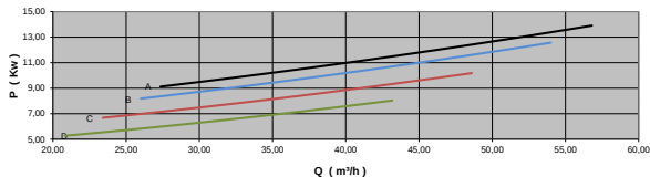
Potenza Ass. / Abs Power ( Kw )
